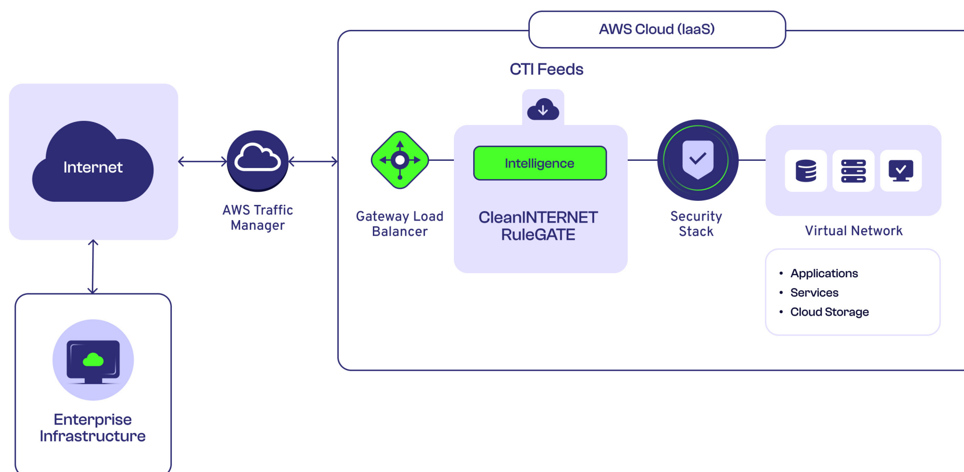
Typical Configuration for Centripetal CleanINTERNET® CLOUD for AWS
